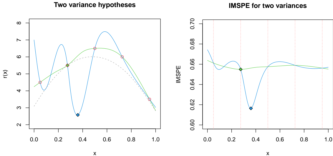
Figure 6: Two hypothetical variance functions (left) and the resulting IMSPE surfaces (right) with corresponding minima marked by diamonds. The dashed grey line represents the replication threshold (left).
